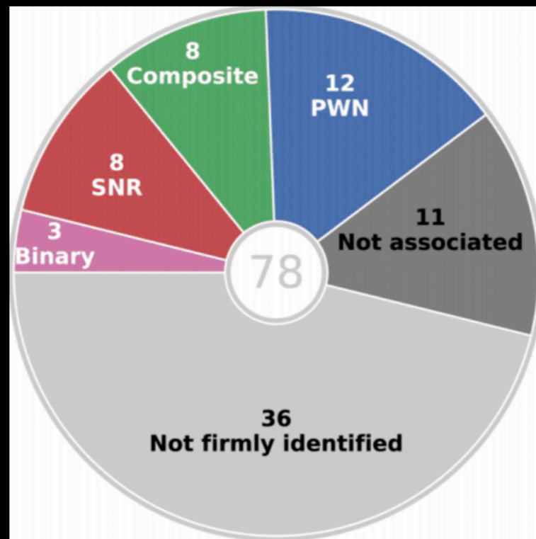
TeV Source Counts
