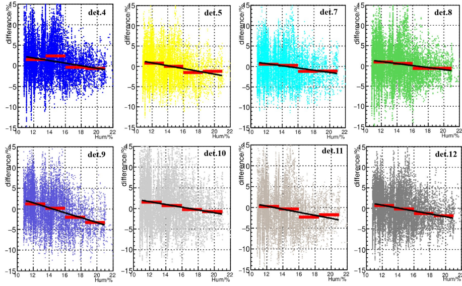
Figure 3: linear fitting of profile of \delta vs humidity of No.1 soil moisture meter
