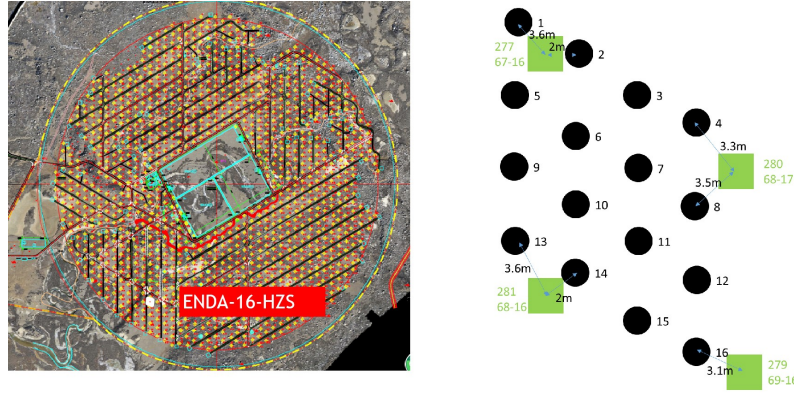
Figure 1: left: Location of ENDA-16-HZS inside the LHAASO. right: Configuration of ENDA-16-HZS. Black circles are EN-detectors; Green squares are EDs.
