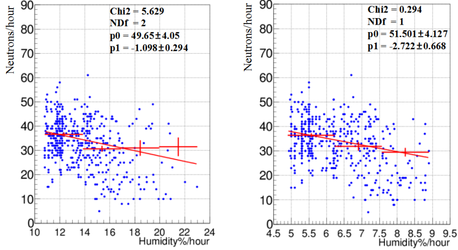
Figure 5: the linear fitting of of scattering plot of neutrons per hour vs humidity in soil
