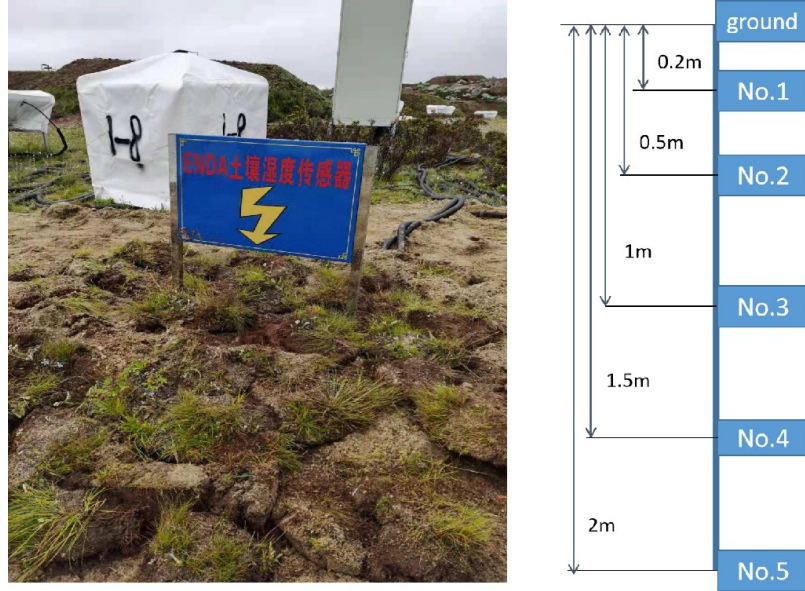
Figure 2: Configuration of soil moisture meters.
