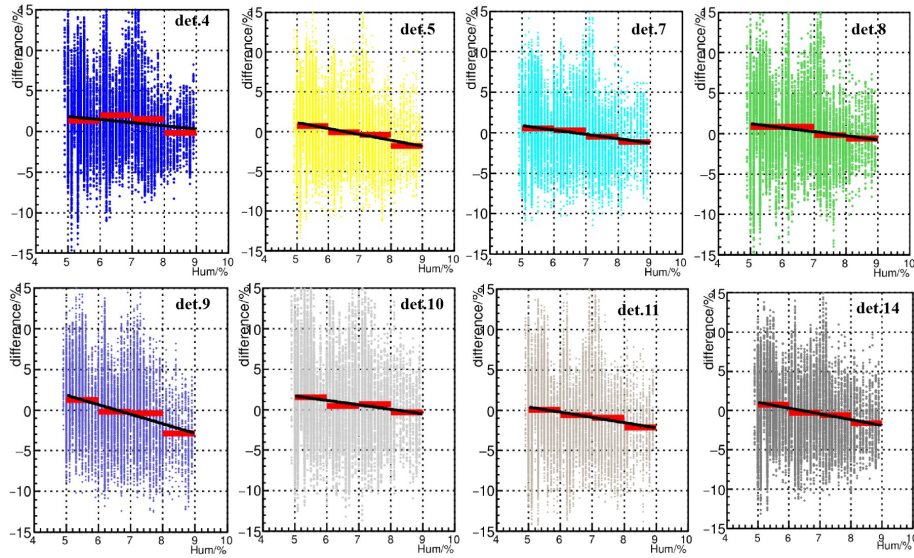
Figure 4: linear fitting of profile of \delta vs humidity of No.2 soil moisture meter
