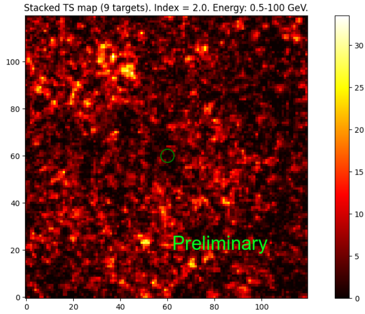
Figure 1: Stacked TS map for the 9 super-luminous stars. There is no hint for collective \gamma -ray emission from this sample in the Fermi -LAT data. The x and y axes are in pixels (the stacked map has no physical coordinates). The color bar represents the TS value.
