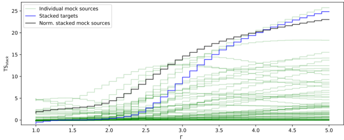
Figure 2: Distribution of TS_{stack} in terms of the photon index \Gamma . The blue line represents the stacked TS for our targets, while the black line represents the normalized stacked background, built with the stacking of 108 mock sources (green lines). Our results are consistent with random background fluctuations. The complete description of this analysis can be found at [8].
